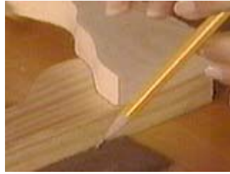
Once the frame is in position, trace the shape of the top piece onto the one below
